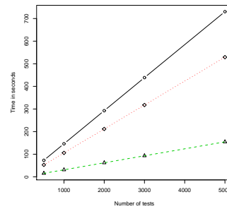
Figure 1: Each point in all graphs corresponds to the average time (over 100 repetitions) for a given number of tests. The horizontal axis is the number of tests. The first row is the G^2 test conditioning on one variable, the second row conditioning on two variables and the third row conditioning on three variables. The green line with the triangle refers to the PLL, the black line with the circle refers to the gSquareDis and the red line with the diamond refers to the disCItest.
